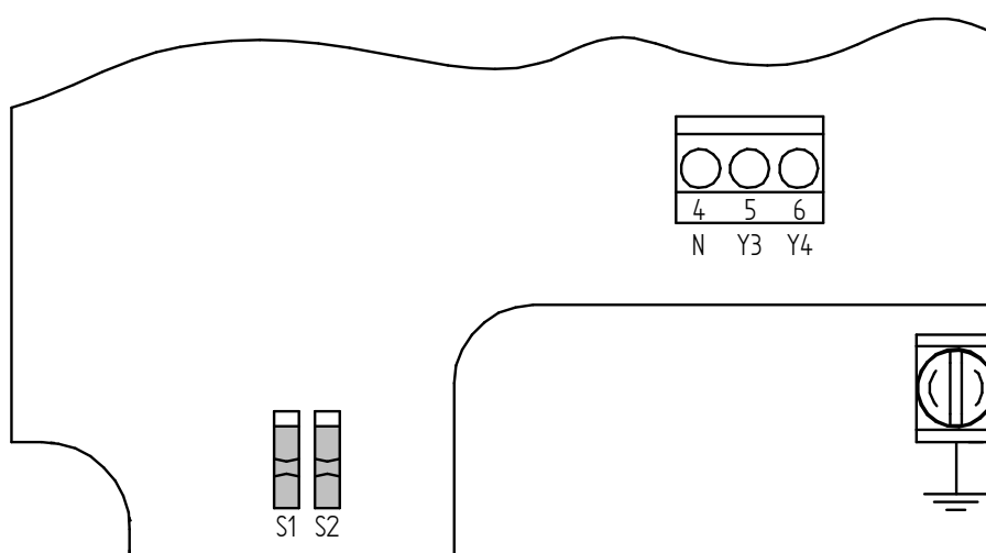
Raccordement 110-240V AC
